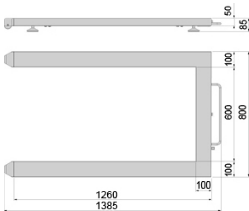
PW: Abmessungen in mm
